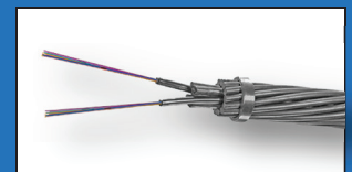
Optical Ground Wire (OPGW)
